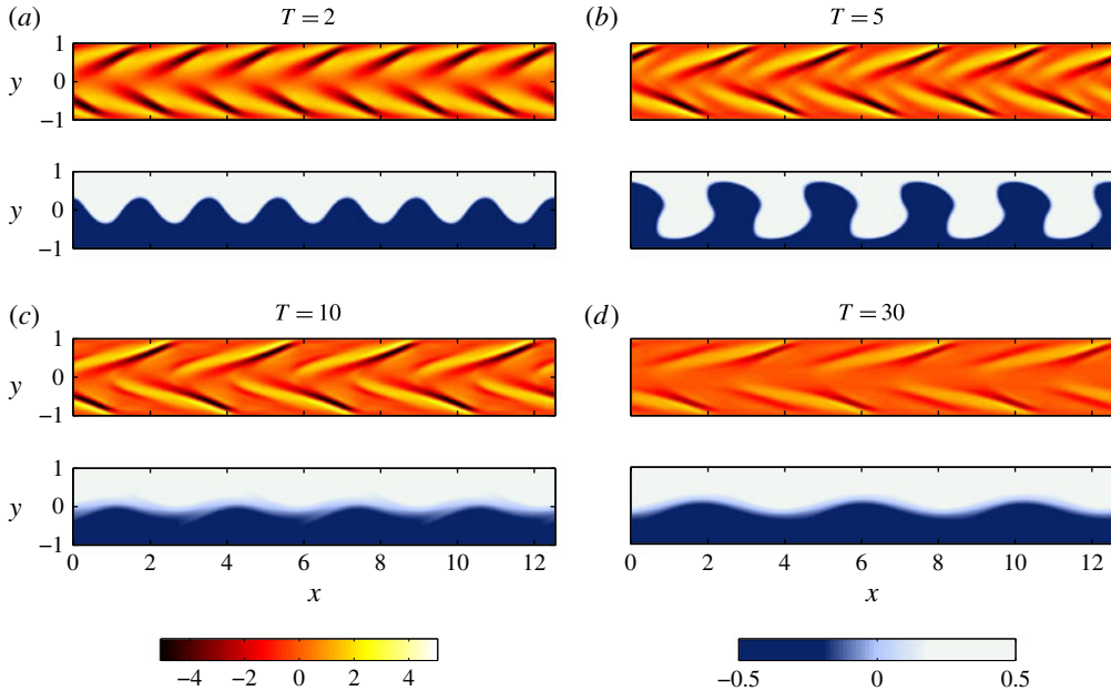
FIGURE 4. (Colour online) Initial vorticity \nabla \times \mathbf{u}_0 (top plot of each pair) and terminal concentration \theta(T) (bottom plot of each pair) distributions corresponding to the time-averaged energy optimisation over the time interval [0, T] for four optimisation times T \in [2; 5; 10; 30] . Colourbars for the vorticity (left) and the concentration field (right) are displayed at the bottom of the figure.
