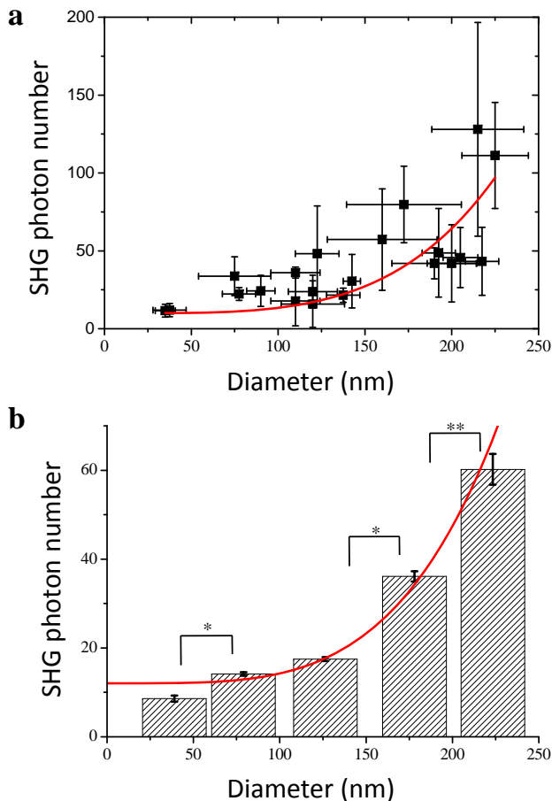
Figure 4. Calibration of collagen SHG signal. SHG photon number as a function of the fibril diameter measured on the TEM image for (a) one sample and (b) all samples using diameter bins of 50 \text{ nm} . Red lines correspond to allometric fitting. The error bar is the standard deviation over 4 measures along 4 different profiles in the same fibril in (a) and the standard error of the mean over all fibrils in the same bin in (b) (6 to 35 fibrils per bin). The symbol * (resp. **) stands for p < 0.05 (resp. p < 0.01 ) using sided two-sample Welch's t-test.
