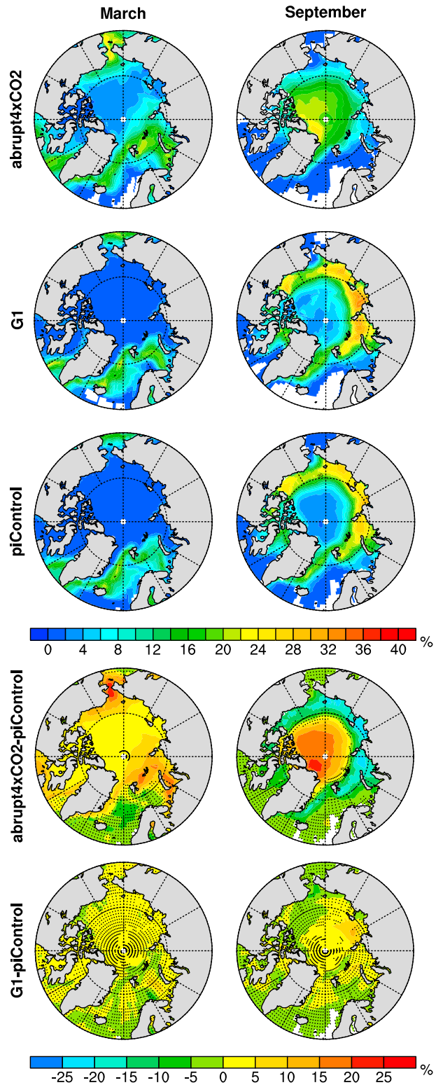
Figure 4. Multimodel ensemble mean standard deviation of March and September sea ice concentration (%) for abrupt4xCO 2 , G1, and piControl and the anomalies for abrupt4xCO 2 -piControl and G1-piControl. Stippling shows where less than six of eight models agree on sign of change. Figure S4 shows the individual model results.
