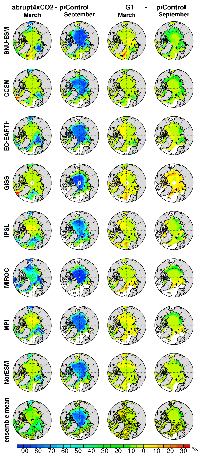
Figure 3. Model simulations of March (maximum sea ice extent) and September (minimum extent) sea ice concentration anomalies (%) for abrupt4xCO 2 -piControl and G1-piControl for the eight models we analyze here. The ensemble mean has stippling where less than six of eight models agree on sign of change. Figure S2 shows the actual sea ice concentration map for each experiment.
