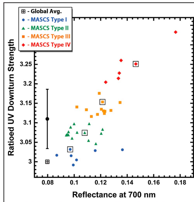
Figure 12. Ratiod UV downturn strength (i.e., UV_{depth} parameter value) versus absolute reflectance at 700 nm for the 39 deposits with MASCS spectral coverage. Note the positive correlation between the UV downturn strength and absolute reflectance at 700 nm ( r^2 = 0.61 ). Plotted reflectance values are an average of three spectral channels centered on ~700 nm in an attempt to reduce spurious results from channel-to-channel instrument noise. Black dot indicates the average UV downturn strength ( \mu_{UV} ); error bars denote \pm 1 standard deviation ( \sigma_{UV} ). Boxes around individual points identify the example spectrum of each type shown in Figure 11.
