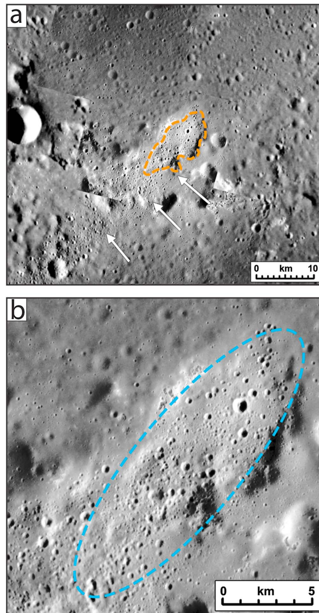
Figure 5. A secondary crater chain from the Hokusai impact crater crosscuts the Praxiteles SW pyroclastic deposit and source vent at 26.0°N, −60.3°E [Kerber et al. , 2011]. North is up in both images. (a) Context image showing the Praxiteles SW pyroclastic deposit and source vent (approximate vent outline is indicated by dashed orange line) and the crosscutting secondary crater chain (indicated by white arrows). Mosaic of MDIS NAC images EN0223745081M, EN0223745074M, and EN0223745067M overlaid on the MDIS-derived global mosaic introduced in Figure 1. (b) Close-up view of the Praxiteles SW pyroclastic deposit source vent. Trend of crosscutting secondary crater chain is indicated by a cyan ellipse. Mosaic of MDIS NAC images EN0223745081M, EN0223745074M, and EN0223745067M.
