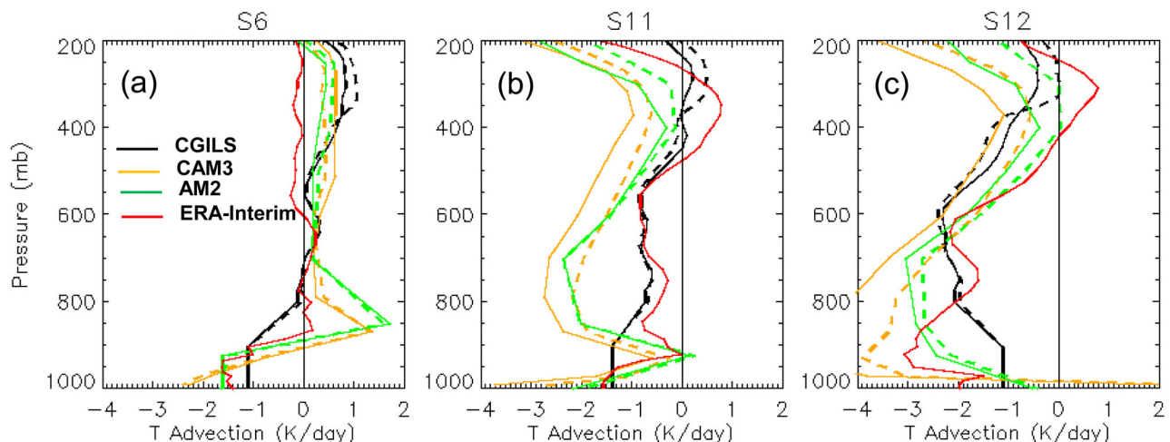
Figure 8. Same as Figure 7 except for horizontal advective tendency of temperature.
