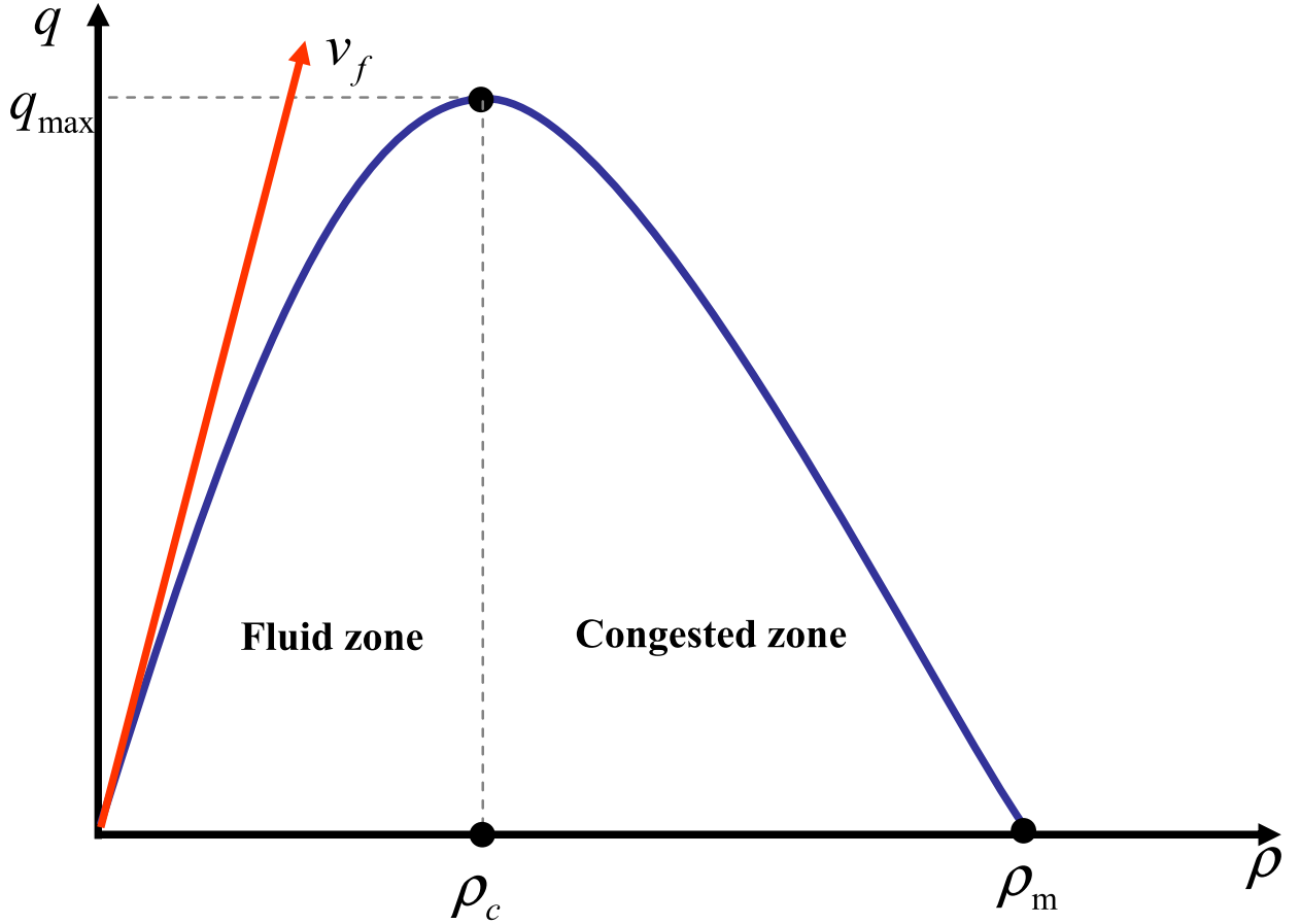
Figure 2. Fundamental diagram: an example
