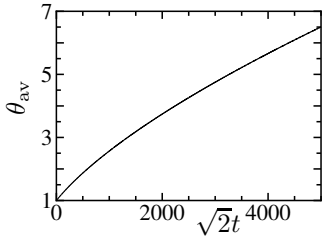
(b) \theta_{av} ( \sqrt{2}t \leq 5000 )
