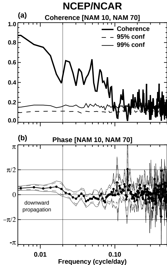
Fig. 1. Cross-spectral analysis between the NAM index at 10 hPa and 70 hPa. Dashed and thin solid lines are the 95% and 99% confidence levels, respectively. The NCEP-NCAR reanalysis.
