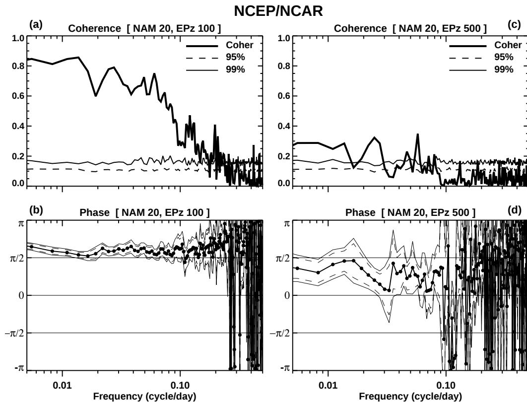
Fig. 3. Cross-spectral analysis between the NAM index at 20 hPa and the vertical EP flux anomalies averaged over 45^{\circ} – 75^{\circ} N at (a, b) 100 hPa, (c, d) 500 hPa. Dashed and thin solid lines are the 95% and 99% confidence levels respectively. The NCEP-NCAR reanalysis.
