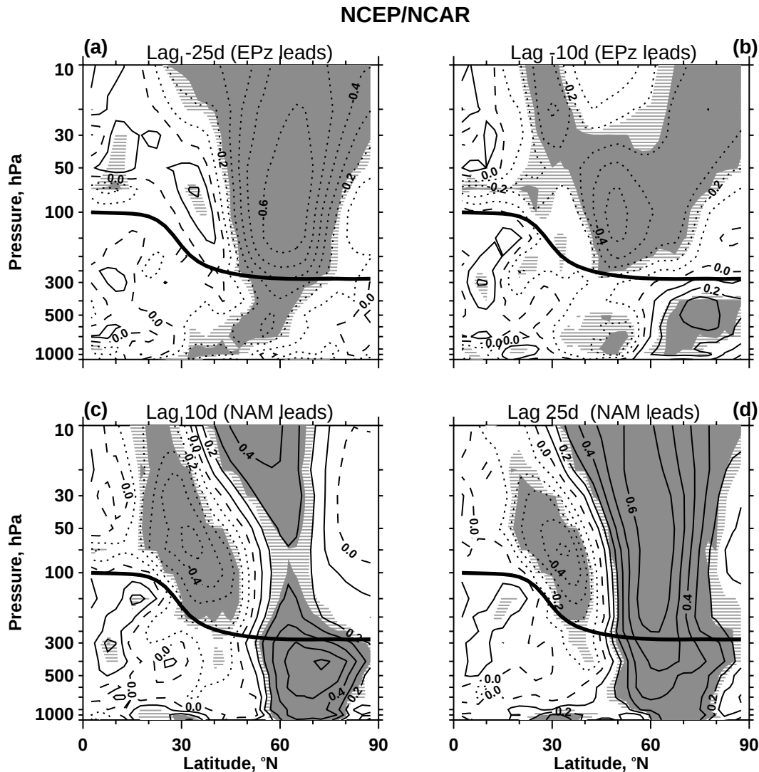
Fig. 7. Cross correlation of the 60-day low-passed NAM index at 20 hPa with the 60-day low-passed vertical EP flux anomalies. Cross-correlations are taken at lags (a) –25, (b) –10, (c) 10 and, (d) 25 days. Contours and shading as in Fig. 2. The NCEP-NCAR reanalysis.
