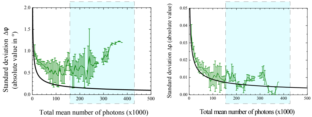
Fig. 6. Precision measurements (— Fit, F-SHG) and theoretical calculation (—) for a Poisson noise. In light blue: usual total mean number of detected photons, considering binning of approx. 400 pixels (for one sub-area) before extracting \varphi and \rho in order to increase measurements accuracy.
