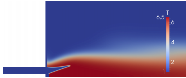
FIG. 7. Base flow used for the linearization procedure, visualized by temperature ratio T/T_u with T_u = 300 K.
