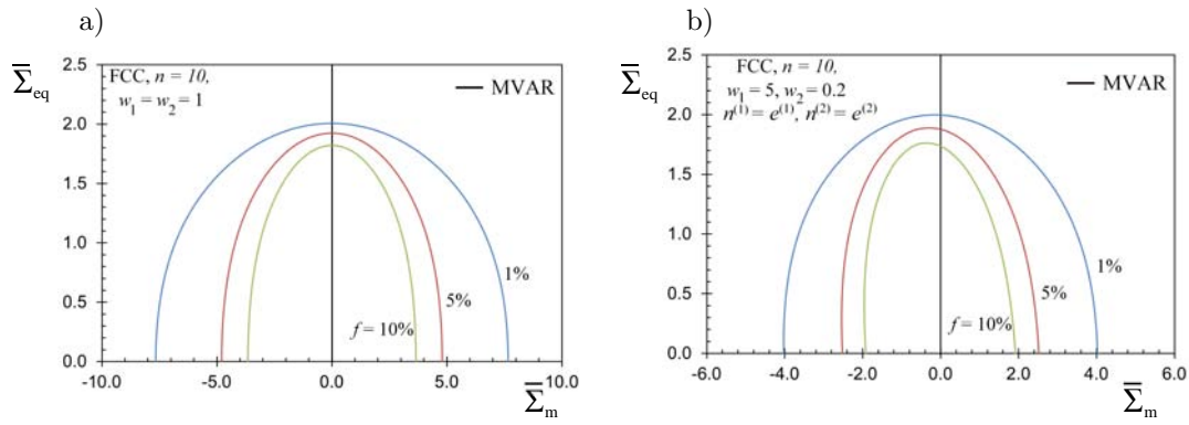
Figure 11: Gauge surfaces in the \bar{\Sigma}_m - \bar{\Sigma}_{eq} plane for a FCC porous single crystal with ellipsoidal voids and a creep exponent n = 10 and a Lode angle \bar{\theta} = 0 . The effect of porosity is investigated by choosing f = (1\%, 5\%, 10\%) for different void shapes (a) w_1 = w_2 = 1 and (b) w_1 = 5, w_2 = 0.2, \mathbf{n}^{(1)} = \mathbf{e}^{(1)}, \mathbf{n}^{(2)} = \mathbf{e}^{(2)} .
