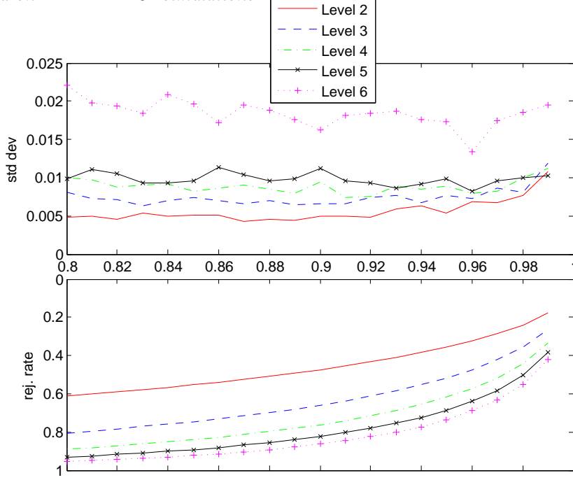
Figure 3.1.2: Adaptive POP method ( p = 10\% ). Standard deviation (std dev.) and corresponding rejection rate (rej. rate), based on 100 macro-runs, of each quantile estimator (\hat{Q}_{N,p}^l)_{1 \leq l \leq L^*-1} and last level occupation measure estimator \hat{r}_N(\hat{Q}_{N,p}^{L_N}) , for different values of \rho .
