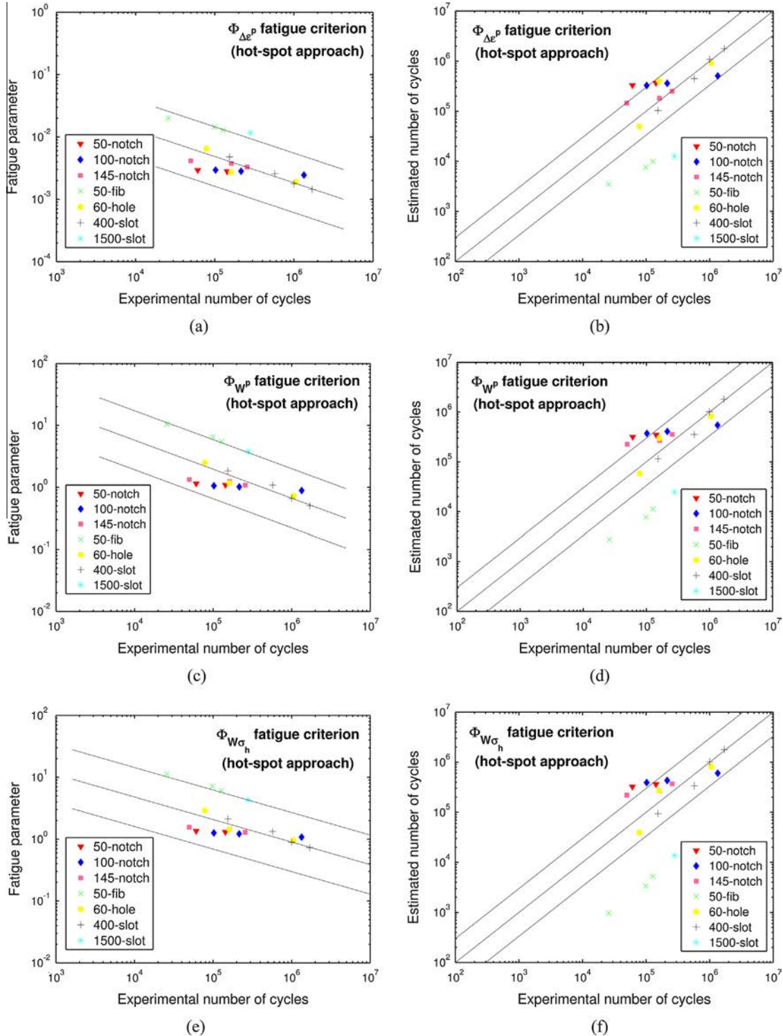
Fig. 14. Hot-spot approach for the \Phi_{\Delta \epsilon^p} , \Phi_{W^p} , and \Phi_{W\sigma_h} fatigue criteria. (a)–(c)–(e) Fatigue parameter vs. experimental number of cycles to failure; (b)–(d)–(f) estimated vs. experimental number of cycles to failure.
