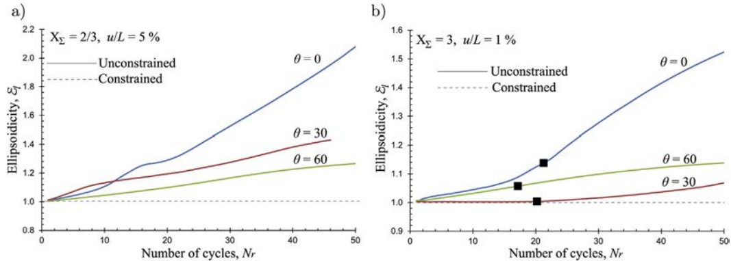
Fig. 17. Ellipsoidicity ratio e_l for an unconstrained void and a spherically constrained void in the case of (a) X_{\Sigma} = 2/3 ( u/L = 5\% ) and (b) X_{\Sigma} = 3 ( u/L = 1\% ) as a function of the number of cycles Nr . The filled square (■) on the graphs indicates the point where maximum equivalent stress is observed.
