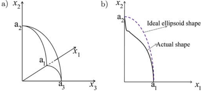
Fig. 5. (a) Schematic representation of 1/8 of the surface of a perfect ellipsoidal void defined by three semi-axes a_i ( i = 1,2,3 ). (b) Cross-section of the void surface in the x_1 - x_2 plane where a representative difference between the actual void shape and an ideal ellipsoid shape having the same aspect ratios.
