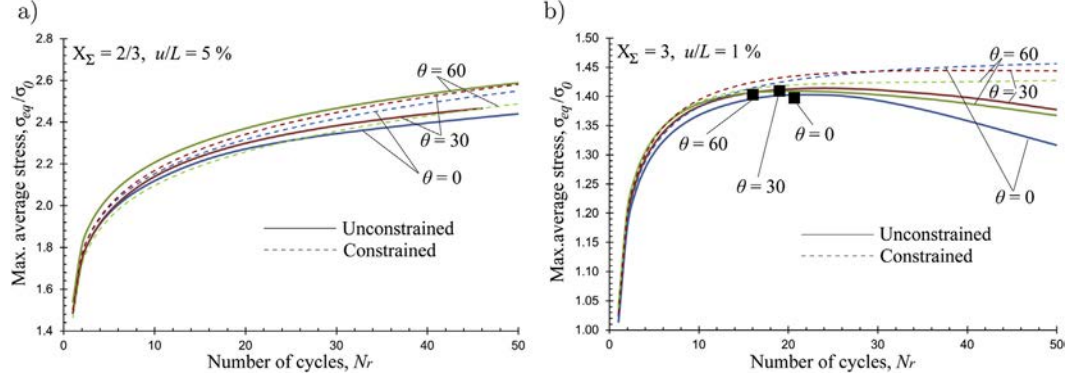
Fig. 13. Normalized maximum average equivalent von Mises stress evolution for unconstrained void/spherically constrained void in the case of (a) u/L = 5\% , X_\Sigma = 2/3 and (b) u/L = 1\% , X_\Sigma = 3 as a function of the number of cycles N_r . The filled square (■) on the graphs indicates the point where maximum stress is observed.
