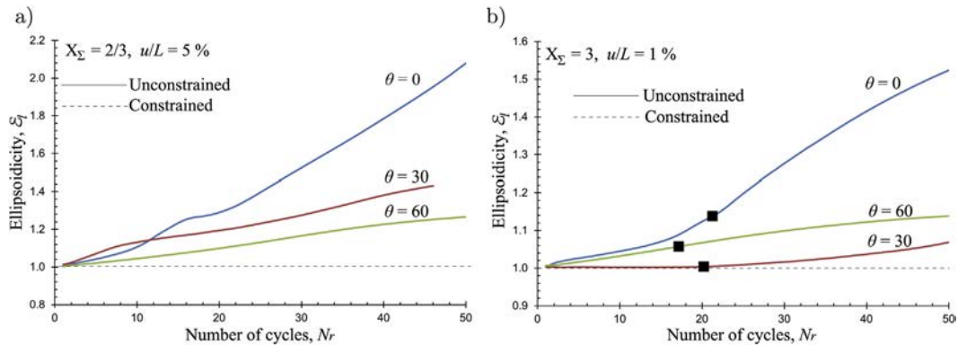
Fig. 17. Ellipsoidicity ratio e_l for an unconstrained void and a spherically constrained void in the case of (a) X_\Sigma = 2/3 ( u/L = 5\% ) and (b) X_\Sigma = 3 ( u/L = 1\% ) as a function of the number of cycles Nr . The filled square (■) on the graphs indicates the point where maximum equivalent stress is observed.
