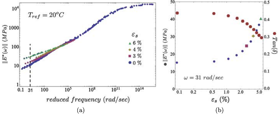
Fig. 5 (a) Complex modulus amplitude master curves under prestrain value \varepsilon_s of 0; 3; 4; 6 % and for a dynamical strain amplitude of \varepsilon_d = 0.02\% and for a reference temperature of T_{ref} = 20^\circ C . (b) Nonlinear evolution of the complex modulus amplitude \|E^*(\omega)\| and the phase angle \delta in function of the prestrain \varepsilon_s for a given angular frequency \omega = 31 rad/s
