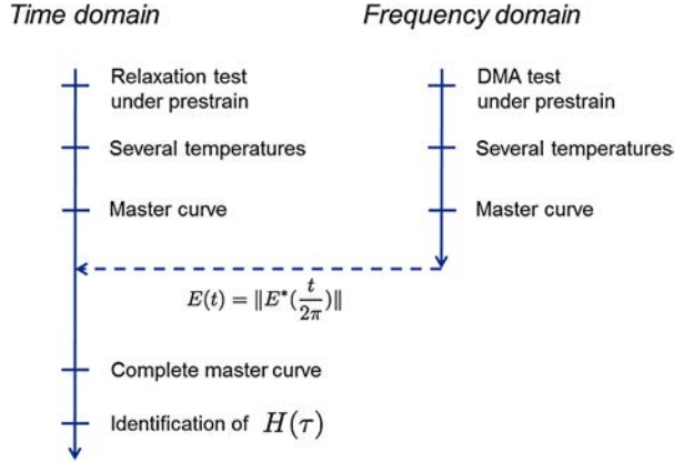
Fig. 2 Schematic view of the experimental procedure
