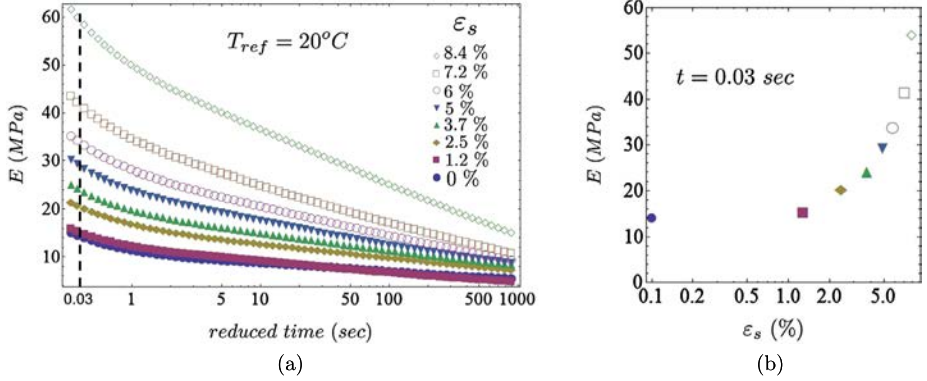
Fig. 4 (a) Relaxation modulus master curves under prestrain between 0\% \leq \varepsilon_s \leq 8.4\% for a relaxation strain step of \varepsilon_0 = 1\% and for a reference temperature of T_{ref} = 20^\circ C . (b) Nonlinear evolution of the relaxation modulus in function of the prestrain \varepsilon_s for a given time t = 0.03 s
