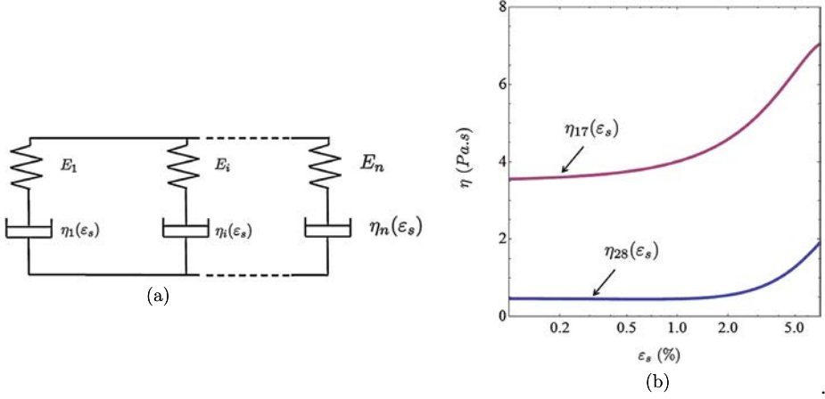
Fig. 11 (a) Schematic view of a generalized Maxwell model with variable, prestrain dependent viscosity. (b) Evolution of viscosity with prestrain in the 17th and 28th element of the identified model
