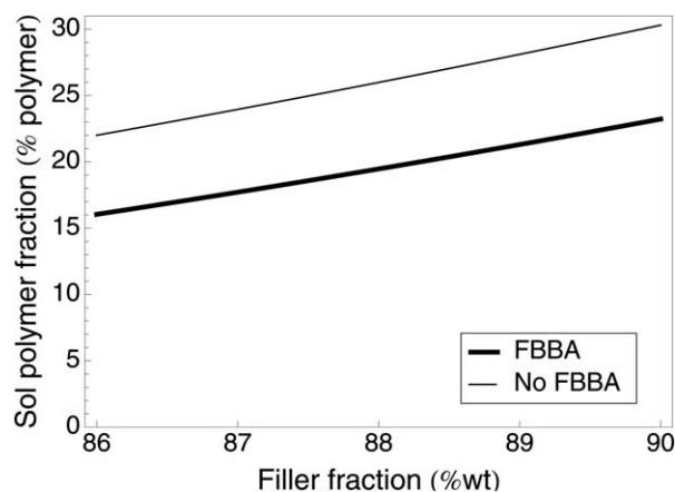
Figure 3. Influence of filler fraction and FBBA on the sol polymer fraction F_{solpol} . NCO/OH = 0.95, plasticizer = 20 wt % of the binder.
