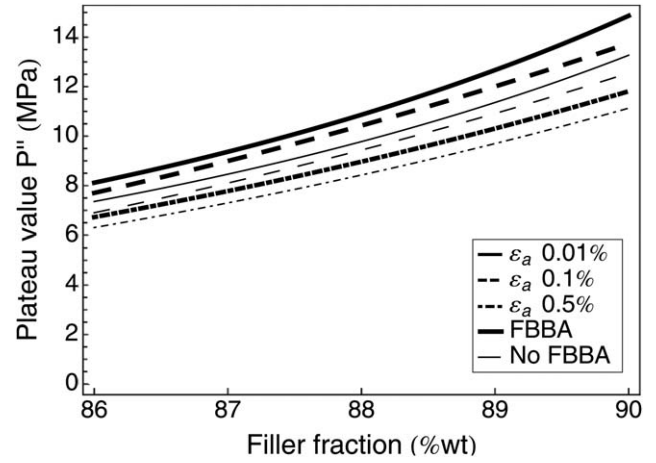
Figure 5. Influence of filler fraction and FBBA on the plateau value P'' . NCO/OH = 0.95, plasticizer = 20 wt % of the binder.
