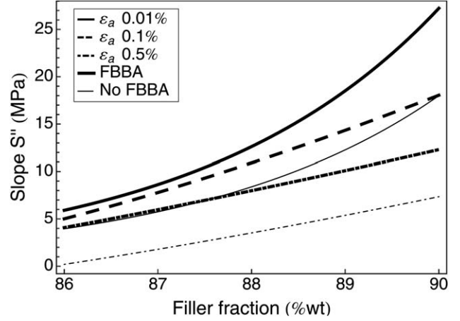
Figure 9. Influence of the filler fraction and FBBA on the nonlinearity slope S'' ; NCO/OH ratio = 0.95, plasticizer = 20 wt % of the binder.
