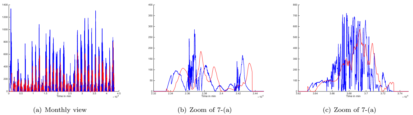
Fig. 7. June : volatility (blue) and its trend prediction (red)
