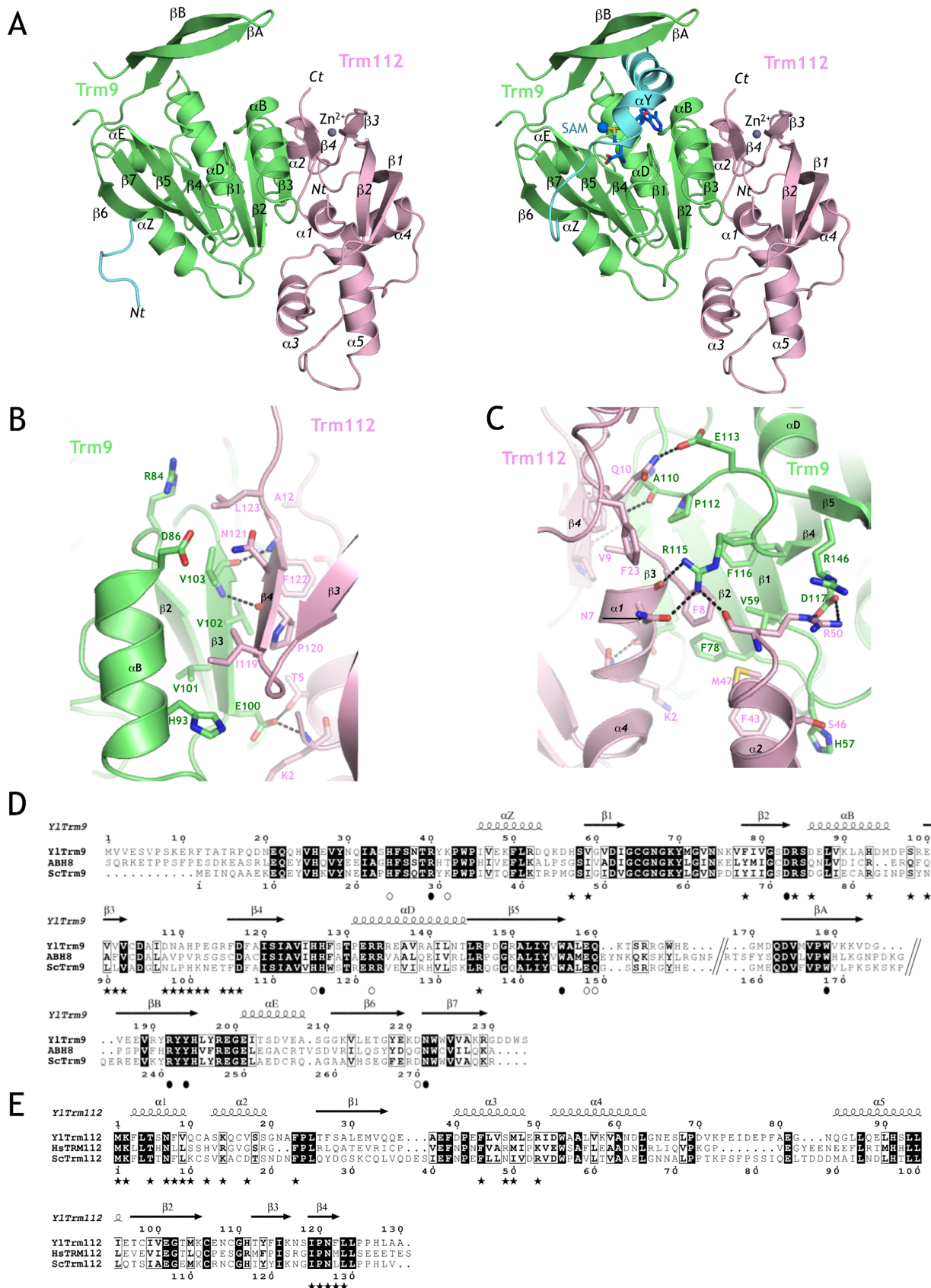
Figure 1. Structure of the YlTrm9 - Trm112 complex. (A) Ribbon representations of the crystal structure of the YlTrm9 N38- Trm112 complex (left) and of the model of the YlTrm9 N20- Trm112 complex (right). On the left panel, residues 39–44, which adopt different conformations between our crystal
