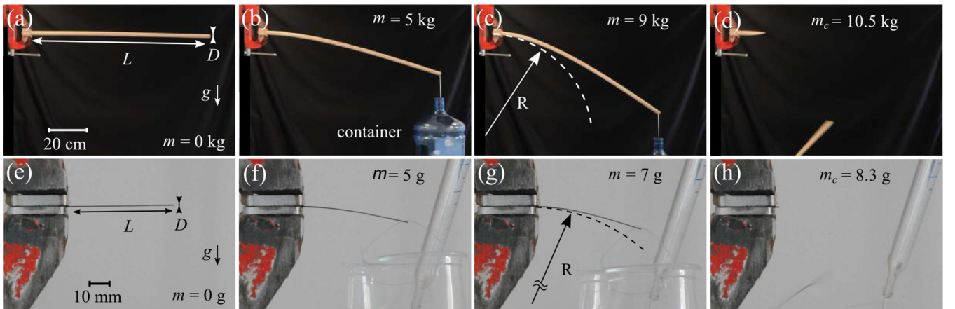
FIG. 3. Deformation of a rod induced by a point mass m suspended at the free end. (a)–(d) Wood rod. (e)–(h) Pencil lead. While the length scales are roughly divided by ten, the mass scale is lowered by a factor one thousand.
