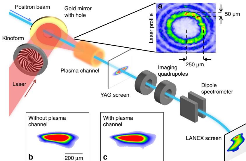
Figure 1 | Experimental layout. The laser passes through the kinoform and is coupled to the beam axis by a gold mirror with a small central hole. Inset (a) shows the laser profile upstream of the lithium oven. A scintillating YAG screen 1.95 m downstream of plasma is used to measure the positron beam profile. Inset (b) shows the positron beam spatial profile as imaged on the YAG screen with the laser off and no plasma present. Inset (c) shows the beam profile with the laser on when the positron beam propagates through the plasma channel. The two profiles are similar, indicating that there are no net focusing forces because of the plasma channel. A scintillating Lanex screen downstream of the dipole measures the beam energy spectrum.
