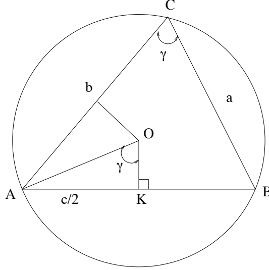
FIGURE 2.3. Triangle ABC
