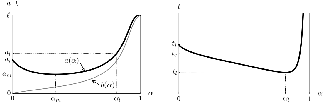
FIGURE 4. Typical dependence of a , b and t on \alpha = b/a . Here the curves correspond to the case where d_c/\ell = 0.1 .
