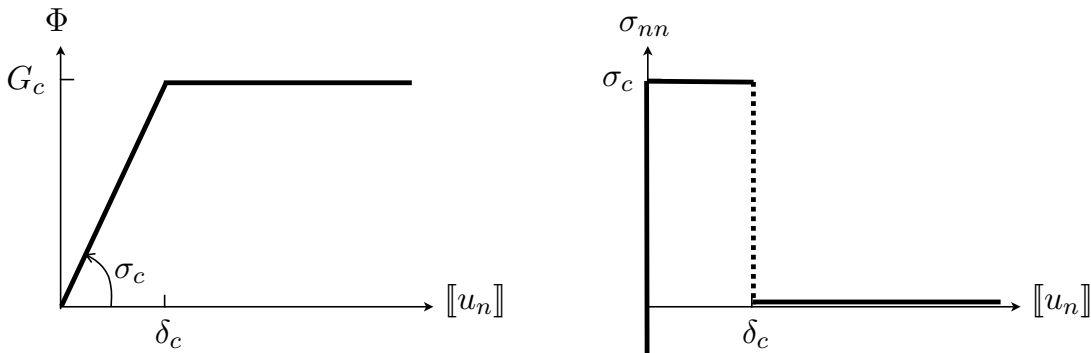
FIGURE 2. Surface energy density and cohesive forces in the model of Dugdale.
