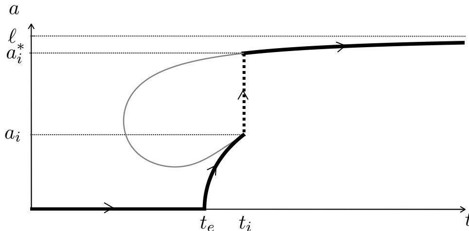
FIGURE 8. Evolution of the crack length under a monotonic increasing loading when d_c/\ell = 0.1 . Note the jump at t = t_i .
