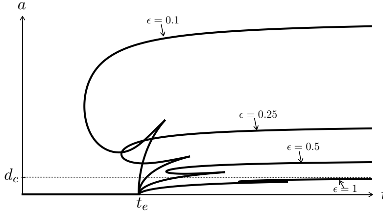
FIGURE 7. Dependence of Dugdale's branches on the stress gradient length \ell = d_c/\epsilon at fixed characteristic material length d_c .
