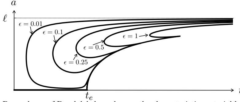
FIGURE 6. Dependence of Dugdale's branches on the characteristic material length d_c = \epsilon \ell at fixed stress gradient length \ell .
