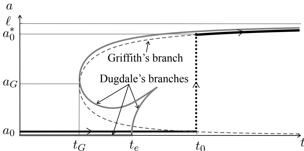
FIGURE 10. Comparison of Dugdale's branches with Griffith's branch when d_c/\ell = 0.1 . In dark, the response associated with Griffith's law under monotonic loading when the body contains an initial crack of half-length a_0 .
