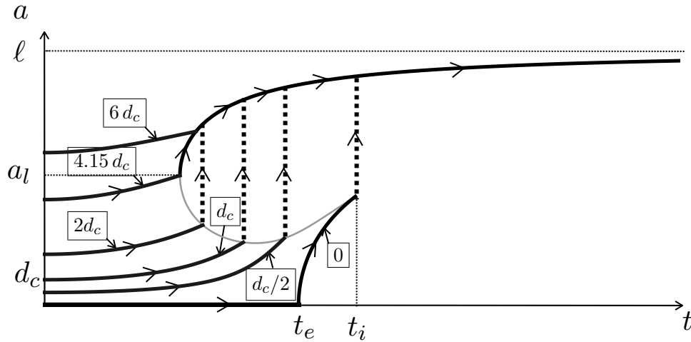
FIGURE 9. Evolution of the crack length a under a monotonic increasing loading for different lengths a_0 of the centered initial non cohesive crack. Here, d_c/\ell = 0.1 and a_0 = 0, d_c/2, d_c, 2d_c, 4.15d_c, 6d_c .
