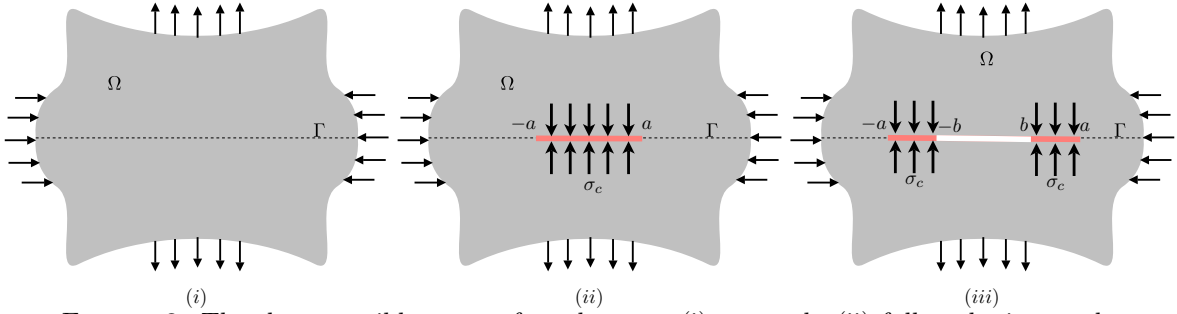
FIGURE 3. The three possible types of crack state: (i) no crack, (ii) fully cohesive crack, (iii) partially non cohesive crack
