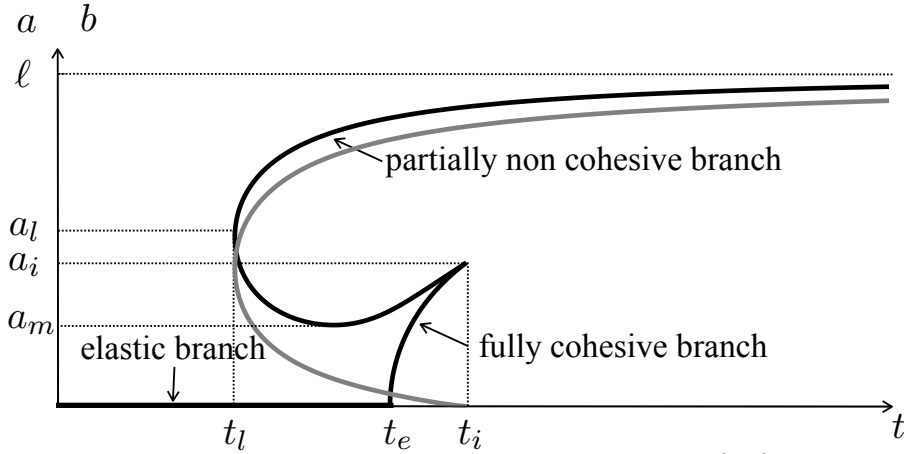
FIGURE 5. Typical graphs of the three branches in the diagram (t, a) . The gray curve represents the evolution of the tip b of the non cohesive crack for the partially non cohesive branch. Here the curves correspond to the case where d_c/\ell = 0.1 .
