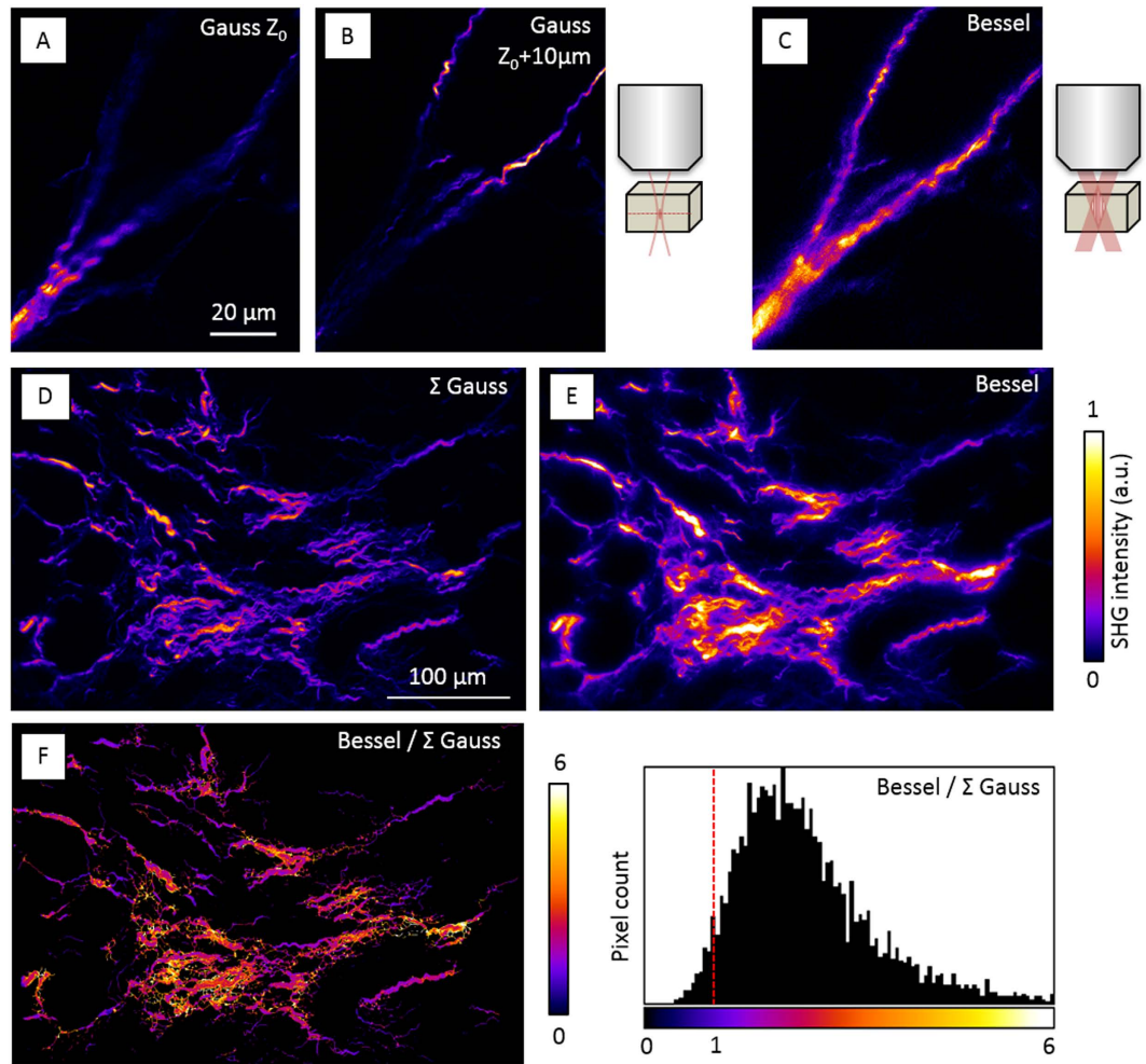
Figure 3. SHG microscopy with axially extended depth of field. (A–C) Images of collagen fibers within a 15 \mu\text{m} thick histological section of mouse kidney were recorded with Gaussian ( 0.7 \mu\text{m} \times 0.3 \mu\text{m} ) and Bessel ( 7 \mu\text{m} \times 0.3 \mu\text{m} ) excitations (800 nm). (A,B) Gaussian 2D images recorded at different depths. (C) 2D image of the same field recorded with Bessel excitation. (D–F) Comparison of SHG imaging contrast using Bessel and Gaussian excitations. (D) image of collagen fibers with 3D-scanned Gaussian excitation ( 0.7 \mu\text{m} \times 0.3 \mu\text{m} ) and sum projection of a Z-series. (E), corresponding field recorded with 2D-scanned Bessel excitation ( 23 \mu\text{m} \times 0.3 \mu\text{m} ) and off-axis detection. (F) Ratio of Bessel-to-Gaussian images calculated assuming similar signals for the smallest fibers. The corresponding histogram is shown on the right. Values superior to 1 reflect the coherent enhancement obtained with extended-depth Bessel excitation. Pixel dwell times, excitation powers after the objective, and maximum signal levels: (A,B) 65 \mu\text{s} , 43 mW, 250 photons; (C) 330 \mu\text{s} , 35 mW, 70 photons; (D) 5 \mu\text{s} \times 20 , 12 mW, 250 photons/plane; (E) 20 \mu\text{s} , 45 mW, 230 photons.
