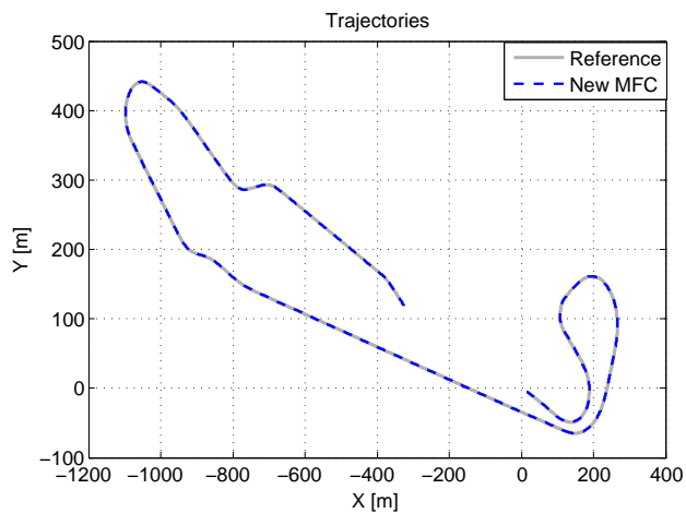
Fig. 15. Reference trajectory versus the simulated closed-loop trajectory
