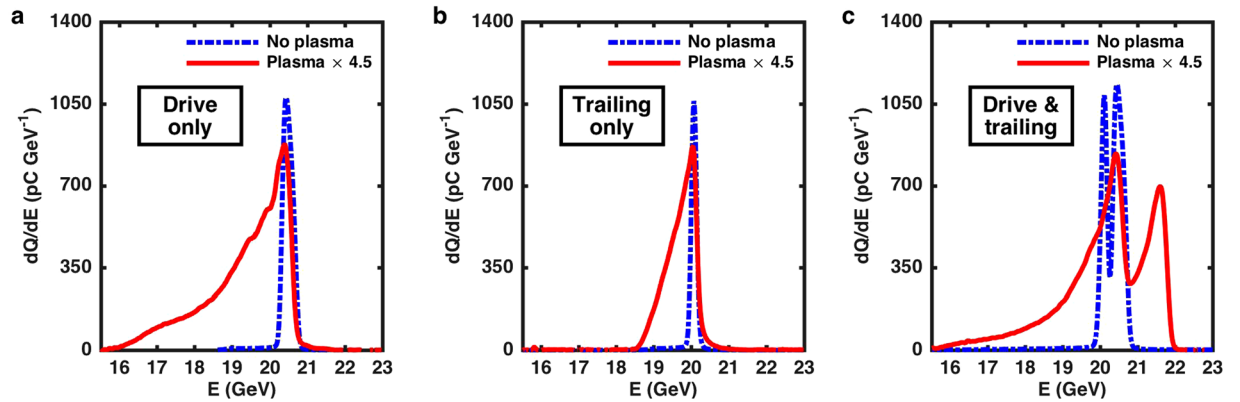
Figure 2. Evidence of acceleration of a positron bunch. Positron energy spectra measured by the Cherenkov energy spectrometer with (red solid line) and without plasma (ionizing laser off, blue dash-dotted line). In (a) only the drive bunch is sent, in (b) only the trailing bunch is sent, and in (c) both the drive and the trailing bunches are sent through the lithium oven, in which case the trailing bunch is accelerated from 20.05 GeV to above 21 GeV by the plasma wake. The plasma data is multiplied by 4.5 in (a–c). The spectrum c with plasma is one of the 160 spectra from the dataset used in Fig. 3.
