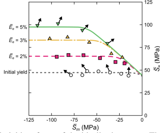
Figure 4: The measured yield surfaces of the idealised cermets. The initial yield surface and the evolution of the surface for 3 additional values of the effective strain \bar{E}_e are included. The plastic strain rate vectors are included for selected loading points with the \dot{\bar{E}}_e and \dot{\bar{E}}_m axes co-incident with the \bar{S}_e and \bar{S}_m axes, respectively.
