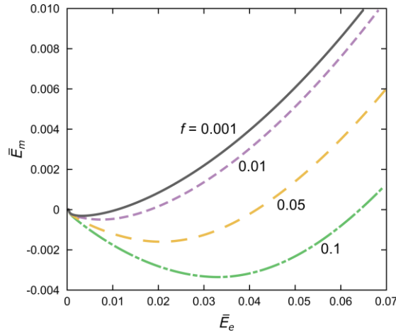
Figure 13: Predictions of the variation of \bar{E}_m with \bar{E}_e for uniaxial compression ( Y = 1/3 ) of the V_f = 0.6 composite with the FCC unit cell. Results are shown for initial matrix porosities in the range 0.001 \leq f_0 \leq 0.1 .
