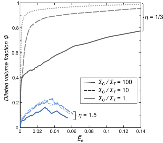
Figure 20: Discrete element predictions of the fraction \phi of the specimen that undergoes dilation, as a function of the macroscopic strain \bar{E}_e for two selected values of the triaxiality \eta . In each case we show results for the reference value of \Sigma_C/\Sigma_T = 1 and two additional values of \Sigma_C/\Sigma_T .
