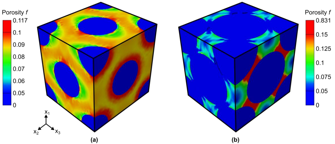
Figure 12: Predictions of spatial distribution of the porosity f in the matrix in the FCC unit cell with volume fractions (a) V_f = 0.2 and (b) V_f = 0.65 of spherical particles. Results are shown for the case of an initial porosity f_0 = 0.1 in the matrix with the unit cell subjected to uniaxial compression ( \gamma = 1/3 ) to a strain \bar{E}_e = 0.1 . Loading is axisymmetric about the x_3 -axis.
