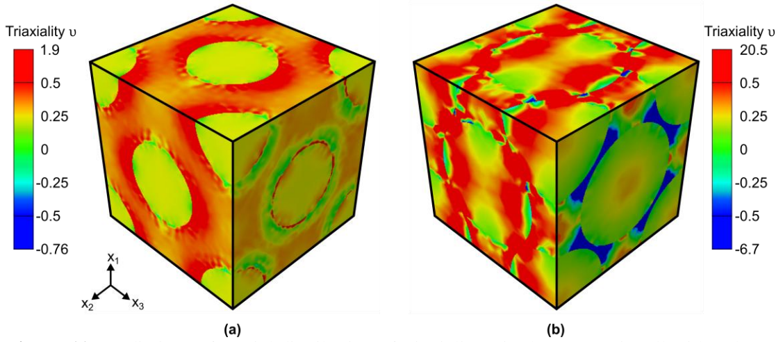
Figure 11: Predictions of spatial distribution of triaxiality v in the FCC unit cell with volume fractions (a) V_f = 0.2 and (b) V_f = 0.65 of spherical particles. Results are shown for the case of an initial porosity f_0 = 0.1 in the matrix with the unit cell subjected to uniaxial compression ( \gamma = 1/3 ) to a strain \bar{E}_e = 0.1 . Loading is axisymmetric about the x_3 -axis.
