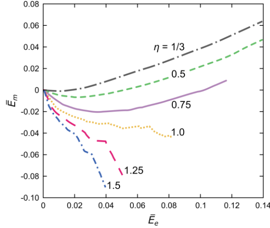
Figure 16: Discrete element predictions of the variation of the macroscopic strains \bar{E}_m and \bar{E}_e for varying levels of triaxiality \eta .
