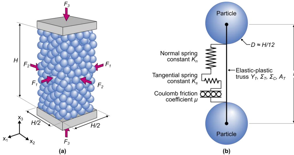
Figure 15: (a) The assembly of 400 spherical particles forming a cuboidal specimen of height H and base H/2 \times H/2 analysed using discrete element simulations. Axisymmetric loading about the x_3 – axis was applied by compressing the specimen between the rigid platens included in the sketch. (b) Sketch of the inter-particle contact model used in the simulations.
