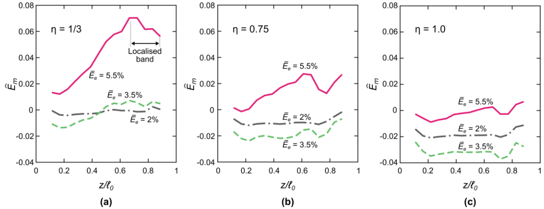
Figure 8: Digital volume correlation (DVC) measurements of the average volumetric strain \bar{E}_m as a function of the normalised axial co-ordinate z/\ell_0 . Measurements are shown for the specimen deformed under stress paths (a) \eta = 1/3 , (b) \eta = 0.75 and (c) \eta = 1.0 for overall strain levels \bar{E}_e = 0.02, 0.035 and 0.055 in each case.
