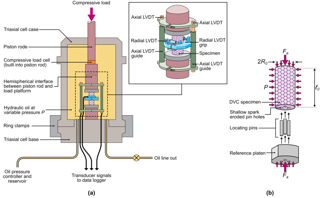
Figure 2: (a) Sketch of the triaxial apparatus used to apply the axisymmetric stress states. The inset shows a magnified view of the specimen with the axial and radial LVDTs used to measure strain. (b) Sketch of the axisymmetric stress state and the three-pin localisation system used to ensure specimen alignment between successive CT scans.
