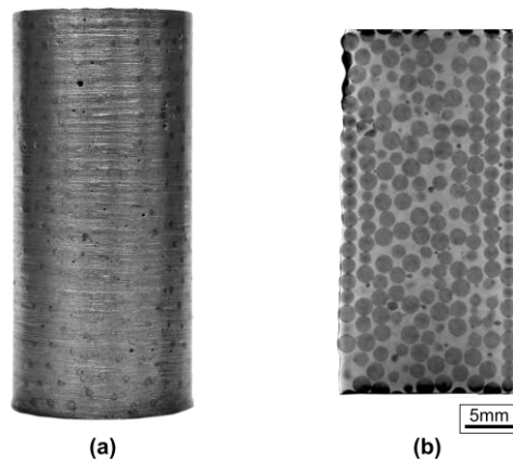
Figure 1: (a) Photograph of the as-cast idealised cermet specimen and (b) a computed tomogram through the centre of the specimen along the longitudinal axis.
