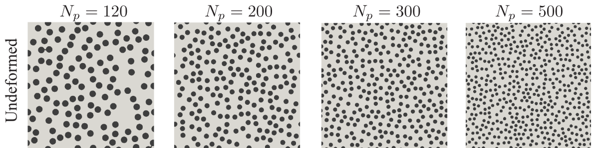
Figure 7: Undeformed unit cells with unstructured isotropic distributions of particles and volume fraction c = 25\text{vol}\% . We show four unit cells with number of particles N_p = 120, 200, 300, 500 .
