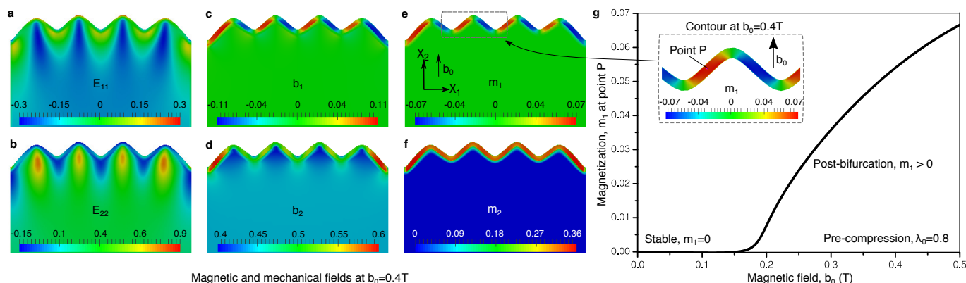
Fig. 6 Numerical post-bifurcation results for the MRE film/substrate system at pre-compression \lambda_0 = 0.8 and b = 0.4\text{T} . Simulation parameters: H_f = 0.8\text{mm} , H_s = 39.2\text{mm} , G_f = 10\text{KPa} , G_s = 3\text{KPa} , \chi_f = 0.4 , \mu_0 m_s^f = 0.5\text{T} . a-f , Deformed configuration and contour plots of the spatial distribution of the Green-Lagrange strains, magnetic fields and magnetization along X_1 and X_2 directions. Part of the substrate is not shown for clarity. g , Supercritical bifurcation curve of magnetization m_1 as a function of the applied magnetic field b_0 , at a fixed point P within the film.
