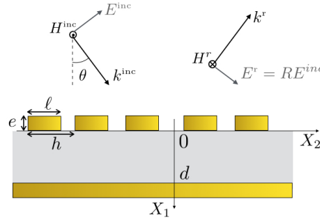
Fig. 3. The scattering problem for the whole metasurface. The reflection coefficient R = -H^r/H^{\text{inc}} is obtained numerically. In the homogenized problem, the metallic array is replaced by the equivalent interface and the propagation in the dielectric slab is explicitly solved.
