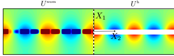
Figure 9: Wavefields of the wave guided within the array; U^{num} computed numerically in the real problem (left panel, X_2 < 0 ), and U^h solution of the homogenized problem, Eqs. (49) -(50) (right panels, X_2 > 0 ). The inclusions are rectangular with e/h = 0.5 and \varphi = 0.9 ; with kh = 0.7 , the wavenumber of the guided wave is \beta h = 1.43 .
