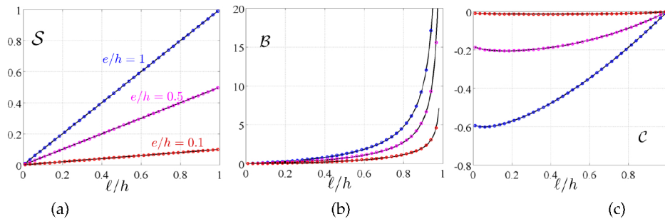
Figure 10. Effective parameters of rectangular Neumann inclusions S, \mathcal{B} and C as a function of \ell/h for e/h = 0.1, 0.5 and 1. Black lines show the interface parameters given by homogenization, Eqs. (3.1) and symbols show the parameters obtained by retrieval method on (R, T) .
