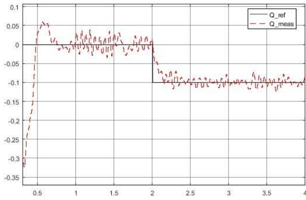
Figure 12. Reactive power response with a multivariable iP ( L_{g1} = 200 \times 10^{-3} )
