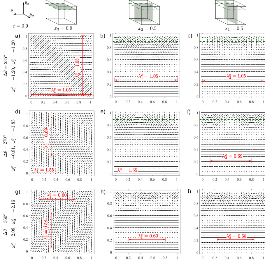
Figure 8: Projections of the post-bifurcated director field \mathbf{n} exhibiting periodic (local) Fredericksz transitions patterns. Different cross-sections of a 5CB-7E bilayer with c = 0.9 under different twist angles \Delta\theta are shown. (a)-(c) \Delta\theta = 235^\circ , (d)-(f) \Delta\theta = 270^\circ and (g)-(i) \Delta\theta = 360^\circ .
