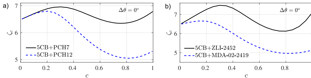
Figure 10: Critical non-dimensional electric field \zeta_c as a function of the bilayer volume fraction c for twist angles \Delta\theta = 0 . Assembly of (a) 5CB-PCH7 and 5CB-PCH12 and (b) 5CB-ZLI-2452 and 5CB-MDA-02-2419 bilayers
