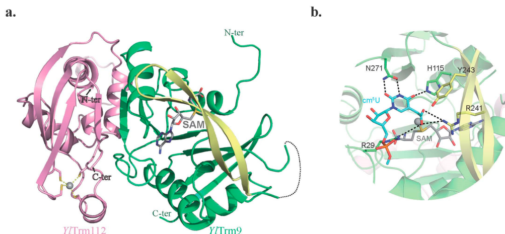
Figure 3. Crystal structure of the Yarrowia lipolytica (Yl) Trm9-Trm112 complex. (a) Ribbon representation of the YlTrm9-Trm112 complex. The S-adenosyl-L-methionine (SAM) molecule (grey sticks), which was absent in the crystal structure, has been modeled by superimposing the SAM-bound structure of Bud23 onto YlTrm9. The Trm9 lid is colored yellow. (b) Model of cm^5U_{34} (blue sticks) docked into the YlTrm9 active site. The SAM methyl group to be transferred is depicted as a sphere. Residues are numbered according to the S. cerevisiae protein.
