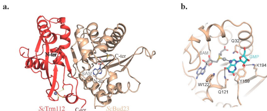
Figure 5. Crystal structure of the S. cerevisiae (Sc) Bud23-Trm112 complex. (a) Ribbon representation of the ScBud23-Trm112 complex bound to SAM. (b) Model of guanosine monophosphate (GMP) (blue sticks) bound to the ScBud23 active site.
