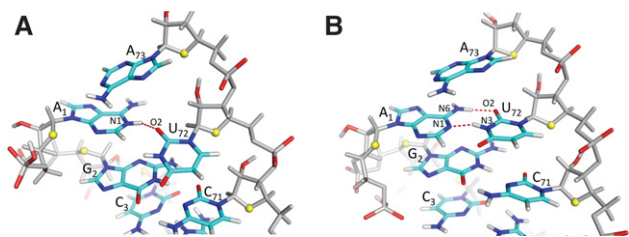
FIGURE 6. Final structures of the \text{A}_1\text{-U}_{72} base pair after 5 nsec of MD simulations of tRNA _f^{\text{Met}}\text{A}_1\text{-U}_{72} in the crystal environment with \text{A}_1 in the N1 protonated form (A) and with \text{A}_1 in the neutral form (B).
