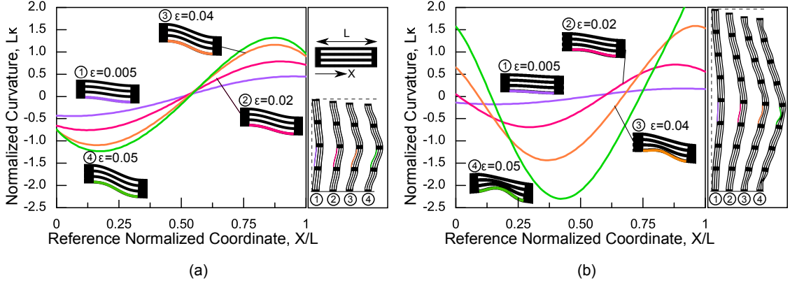
Figure 13: Curvature localization in the hierarchical beams of Fig. 12b and comprised of (a) N_m = 4 and (b) N_m = 8 modules respectively. Plots of the normalized curvature L\kappa as a function of the reference normalized coordinate X/L (see inset) are reported for a selected elemental beam whose profile is extracted from the numerical deformation patterns. For each system, the selected beam is highlighted using coloured lines.
