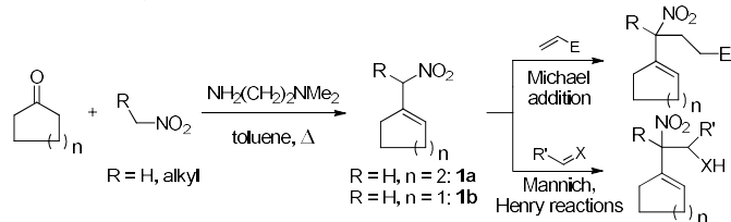
Scheme 2 Nitrocycloalkenyl synthetic platform
