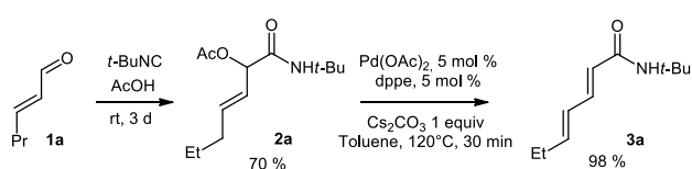
Scheme 2. Passerini/Tsuji-Trost tandem towards diene 2a .
