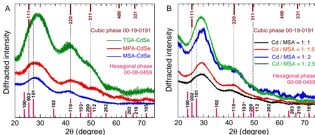
Fig. 3. X-ray diffraction spectra of CdSe QDs capped with three thiol ligands (A) and with different Cd/MSA ratios in the range 1/1 – 1/2.5 (B). The diffraction patterns of cubic and hexagonal phases for bulk CdSe are indicated (from Joint Committee on Powder Diffraction Standards).
