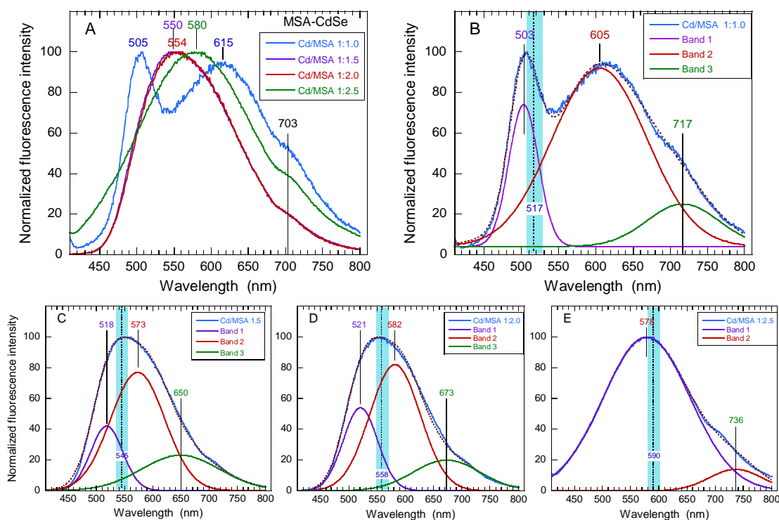
Fig. 6. Fluorescence emission spectra of MSA-CdSe QDs synthesized with different Cd/MSA ratios (A). \lambda_{ex} = 350 nm. [QDs] = 0.05 to 0.15 \text{mg}\cdot\text{mL}^{-1} . Optical pathlength = 1 cm. T = 20 °C. The four spectra of MSA-CdSe QDs were fitted to the sum of three (B, C and D) or two (E) gaussian functions.
