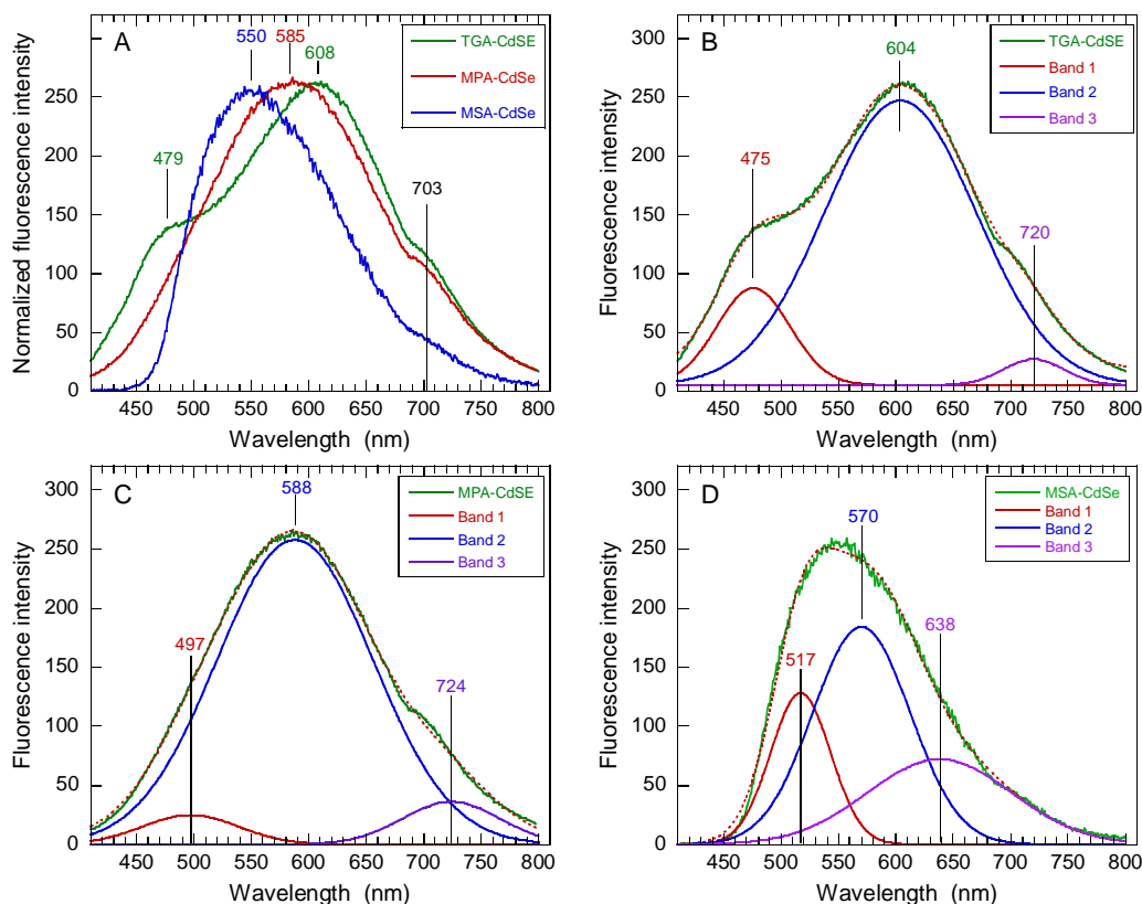
Fig. 5. Fluorescence emission spectra of TGA-, MPA- and MSA-CdSe QDs synthesized with different capping ligands (A). \lambda_{\text{ex}} = 350 nm. [QDs] = 0.05 \text{ mg}\cdot\text{mL}^{-1} . Optical pathlength = 1 cm. T = 20 °C. The three spectra of CdSe QDs were fitted to the sum of three gaussian functions (B, C and D). The red dotted line is the result of the fit.
