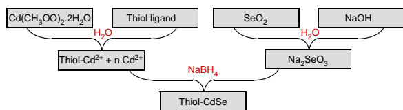
Fig. 1. Summary of the main steps for the synthesis of the capped CdSe nanoparticles. Thiol ligand formulas are given in Scheme 1.
