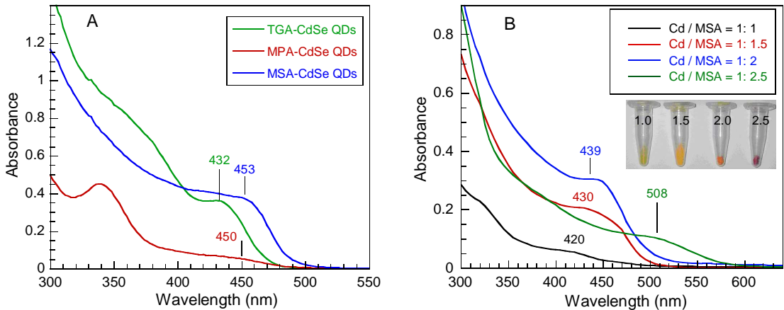
Fig. 4. Electronic absorbance spectra of CdSe QDs synthesized with different capping ligands (A) and with different Cd/MSA ratios (B). [QDs] = 0.05 \text{ mg}\cdot\text{mL}^{-1} for TGA- and MPA-CdSe. [QDs] = 0.05 to 0.15 \text{ mg}\cdot\text{mL}^{-1} for MSA-CdSe. Optical pathlength = 1 \text{ cm} . T = 20 \text{ }^\circ\text{C} .
