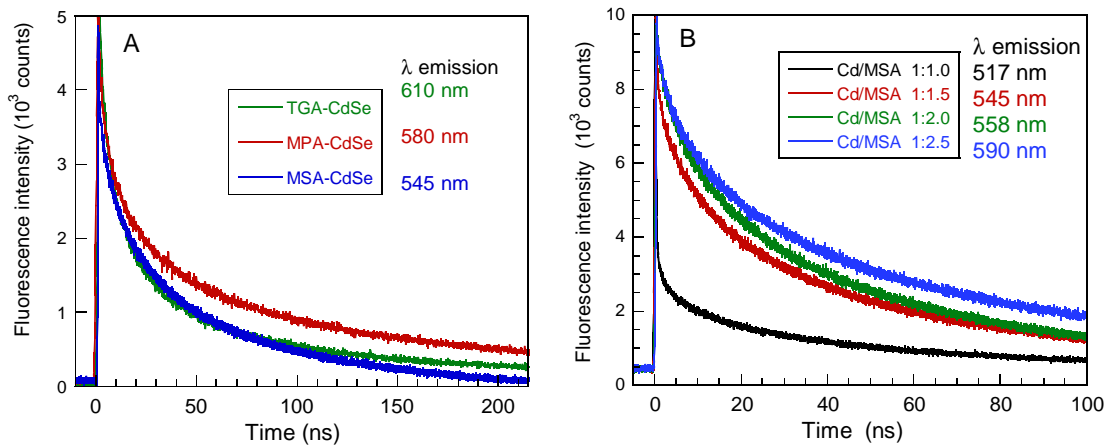
Fig. 7. Time-resolved fluorescence decays of CdSe QDs synthesized with different thiol ligands ( A ) and with different Cd/MSA ratios ( B ). Decays were recorded at the indicated emission maxima. Excitation wavelength \lambda_{ex} = 372 nm. Optical pathlength = 1 cm. The slit width for the emission was set at 25 nm (see Fig. 6).
