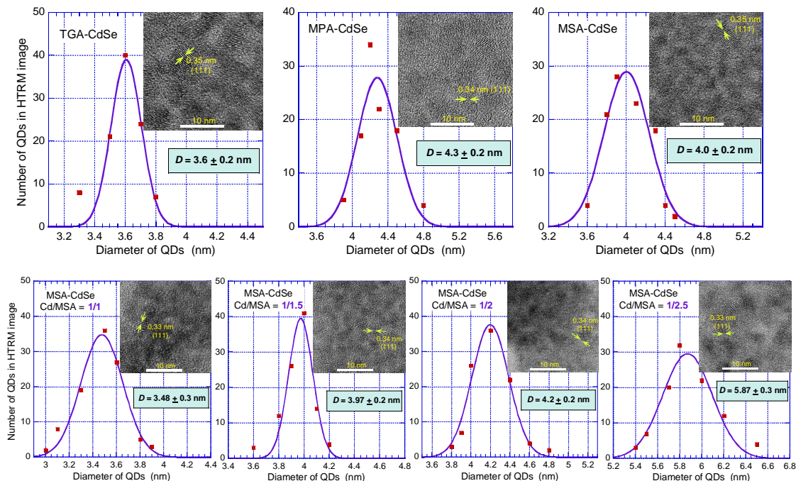
Fig. 2. Gaussian distribution of the size of various synthesized CdSe QDs, with different thiol ligands and different Cd/MSA ratios, determined from individual measures of n = 100 QDs. The insets show the corresponding HRTEM images of CdSe nanocrystals with distinct lattice fringes appearing in one or more directions.
