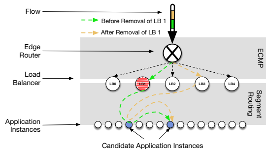
Figure 2. 6LB consistent hashing: when a flow is rebalanced to another load-balancer instance by the edge router, consistent hashing (section III) allows the flow to re-browse the same set of candidate instances, then to be re-pinned to the one that had accepted the connection (section IV).
