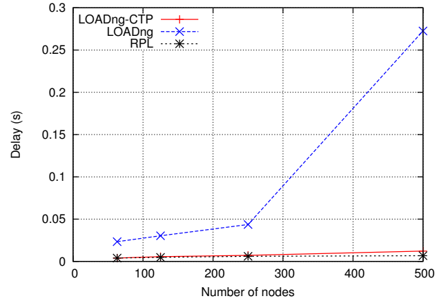
Figure 9: Average end-to-end delay
