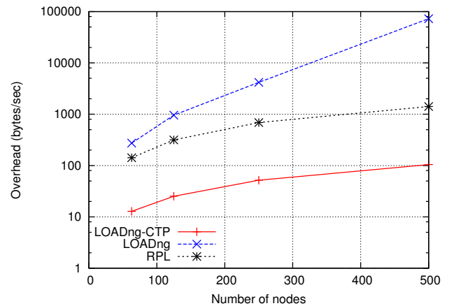
Figure 11: Overhead bytes per second in the whole network
