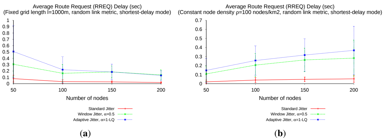
Figure 12. Route discovery delay, shortest-delay RREQ flooding. (a) Fixed grid; (b) Constant router density.
