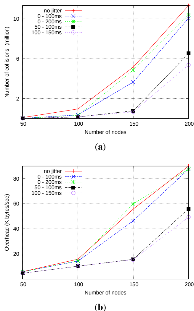
Figure 16. Simulation results of shortest-path RREQ forwarding. (a) Number of collisions; (b) Average overhead.
