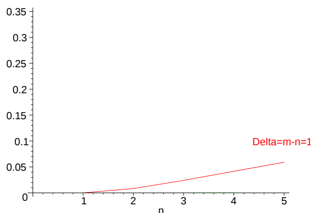
Figure 6. Value of P_W \equiv Pr(D_W^{(n,m)} > 0) , depending on \Delta = m - n > 0 , for different values of n ( \alpha = \frac{1}{2} ). Traces corresponding to \Delta = 2 and \Delta = 3 are significantly lower than 0.01 and, thus, are not visible in the picture.
