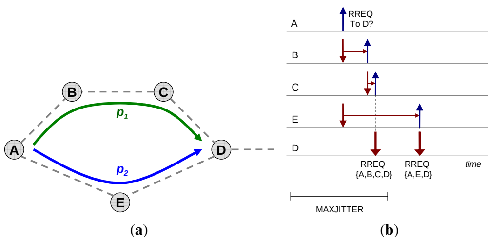
Figure 2. Delay inversion example. Router A tries to broadcast an route request (RREQ) message through the network, through paths p_1 and p_2 . The RREQ through the longer path \{A, B, C, D\} travels faster than the one through the shorter path \{A, E, D\} , due to (unfortunate) jittering. (a) Topology; (b) Example of jitter value assignment for an RREQ from A towards D .
