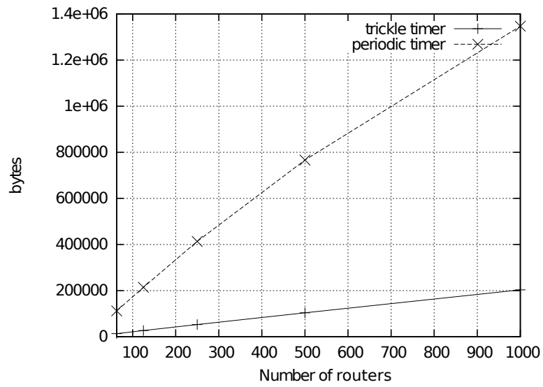
Figure 11: Control traffic: overhead in bytes
