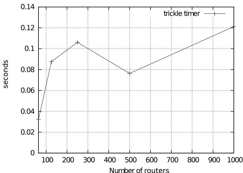
Figure 15: Unicast: delay
