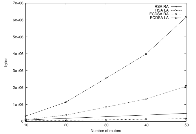
Fig. 4. Total overhead incurring due to signature inclusion.
