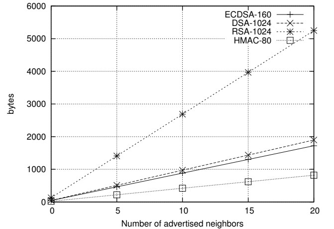
Fig. 5. Link admittance control: Signature overhead per control message with increasing number of advertised neighbors.
