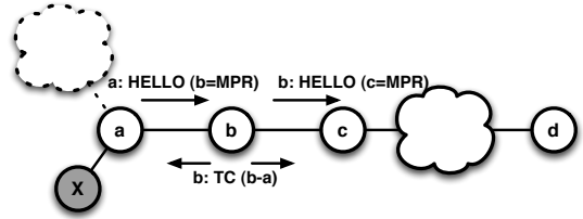
Figure 1. Basic OLSRv2 Operation
