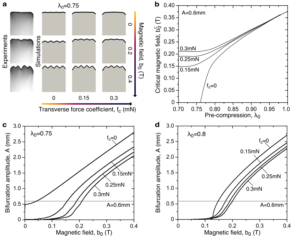
Figure 7: (a) Qualitative comparison of experimental (left column) and numerical (right column) profiles. The effect of friction as measured by the transverse force f_2 = f_c(\lambda_0 - 1) on the lateral faces of the film-substrate block is shown for the numerical calculations. Increase of f_2 delays and even eliminates initial mechanical wrinkling. (b) Effect of friction on the numerical critical magnetic field, b_0^c , and applied pre-compression \lambda_0 map. Numerical bifurcation amplitude response for different transverse force coefficients f_c for (c) \lambda_0 = 0.75 and (d) \lambda_0 = 0.8 as a function of the applied magnetic field b_0 . The dashed line indicates the threshold used to reconstruct the map in part (b).
