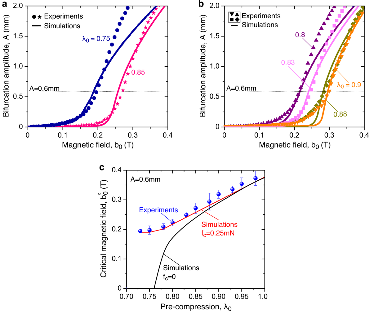
Figure 9: Experiments vs. numerical simulations. (a-b) Bifurcation amplitude curves as a function of the applied magnetic field, b_0 , for various pre-compressions, \lambda_0 . (a) The two curves shown are used for the identification of the MRE shear modulus and friction force f_2 . (b) Comparison between numerical predictions and experiments. (c) Two-field map, \lambda_0 - b_0^c , showing the numerical predictions with ( f_2 = 0.25 mN) and without ( f_2 = 0 mN) lateral friction forces.
